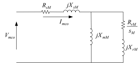
Fig. (4) Per-phase equivalent circuit of an induction motor.
